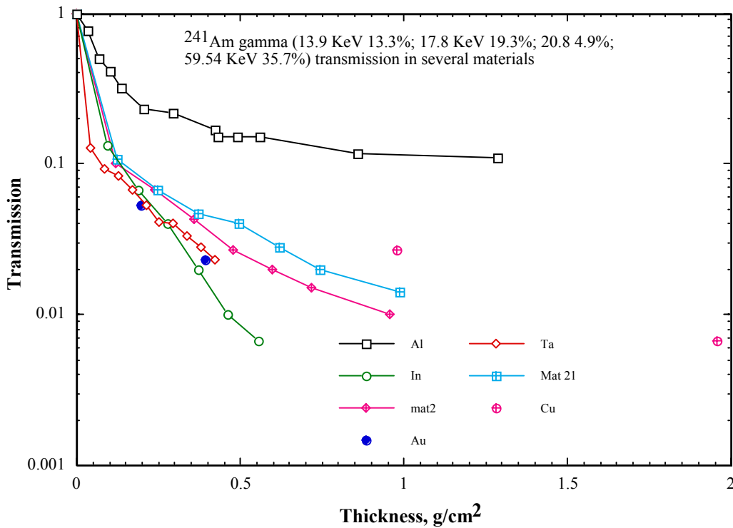
Figure 2. Transmission 241 Am radiation dose through different materials. Results are plotted as a function of surface density.
